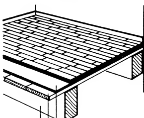
⑭ Finished parquet elements on timber battens
